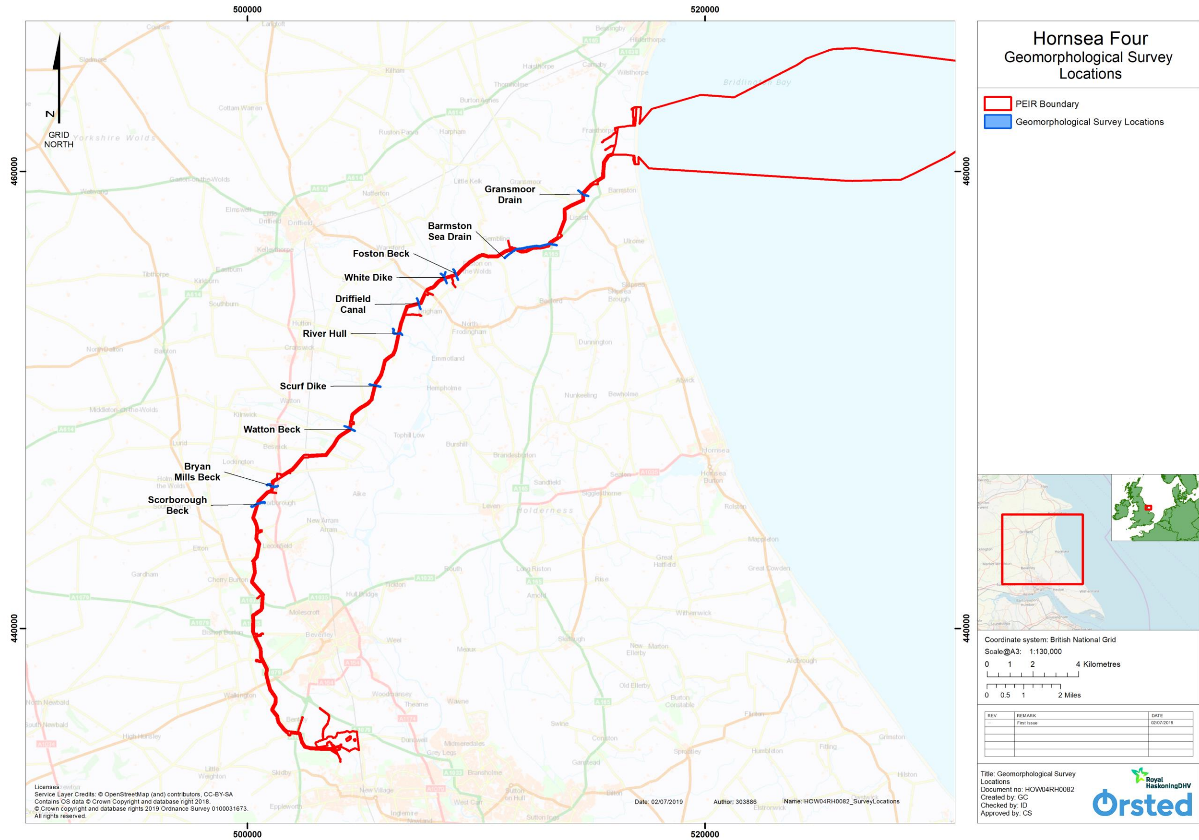
Figure 1: Geomorphological walkover survey study area (Not to Scale).
