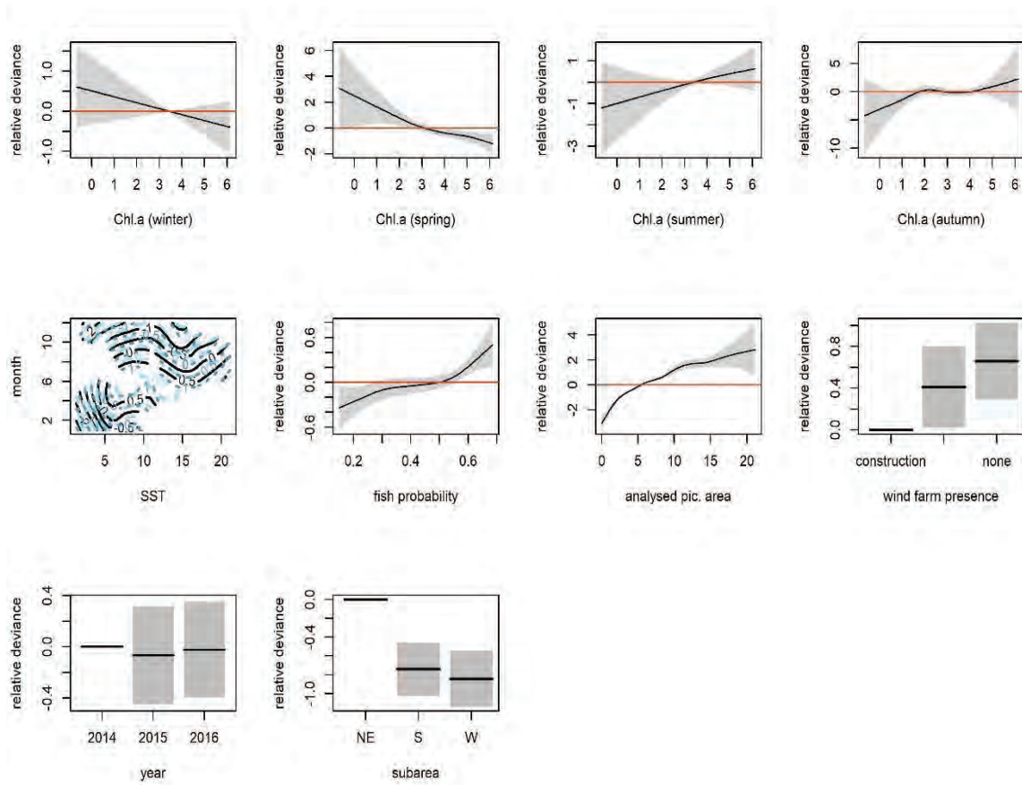
Figure 4.38 Smoothed model parameters for the holistic GAM model of porpoise presence/absence.
