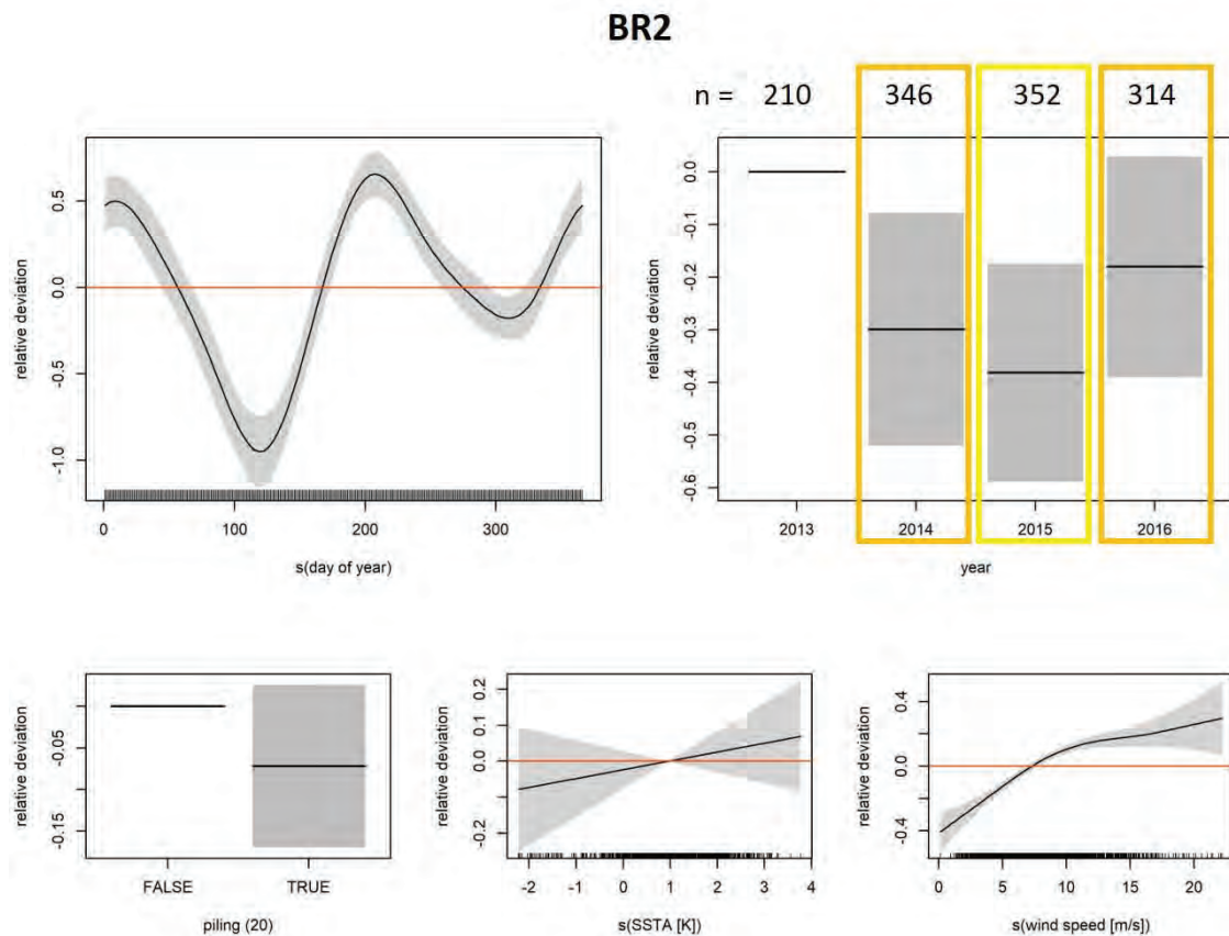
Figure 6.11 Effects of day of year, year, piling at a distance of 20 km, SSTA and wind speed on porpoise detection at the station BR2. Grey-shaded areas indicate the confidence intervals. The number of recording days per year is indicated (n). Years in which piling occurred within a radius of 20 km to the monitoring station are marked with an orange box, years where piling occurred only within a radius of 50 km are marked with a yellow box.
