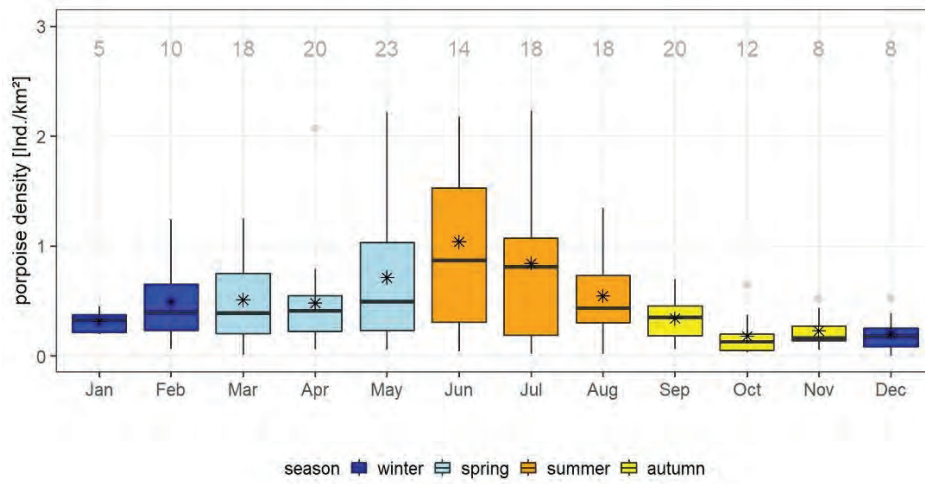
Figure 3.11 Monthly mean porpoise densities [Ind./km 2 ], pooled over the entire study area and study period. Number of flights per month is given in grey.
