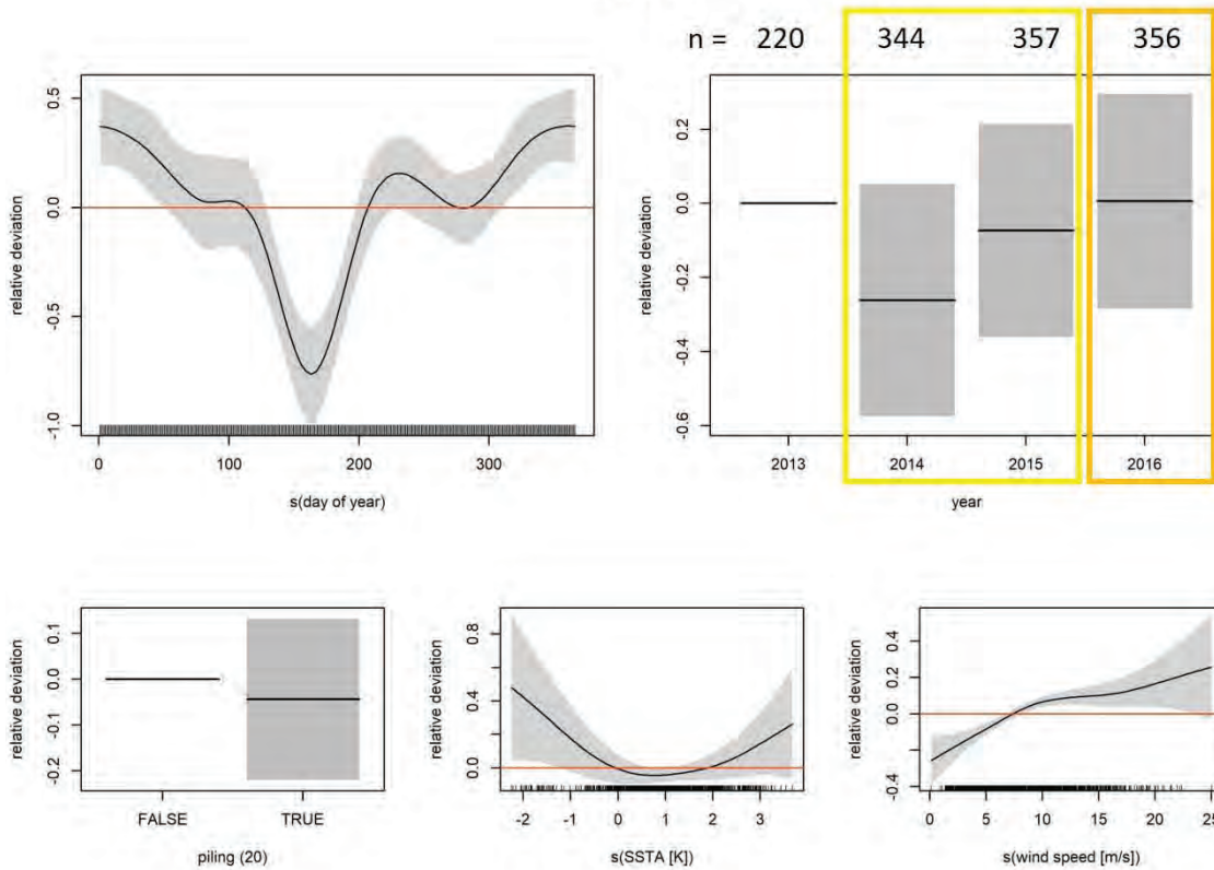
Figure 6.10 Effects of day of year, year, piling at a distance of 20 km, SSTa and wind speed on porpoise detection at the station BR1. Grey-shaded areas indicate the confidence intervals. The number of recording days per year is indicated (n). Years in which piling occurred within a radius of 20 km to the monitoring station are marked with an orange box, years where piling occurred only within a radius of 50 km are marked with a yellow box.
