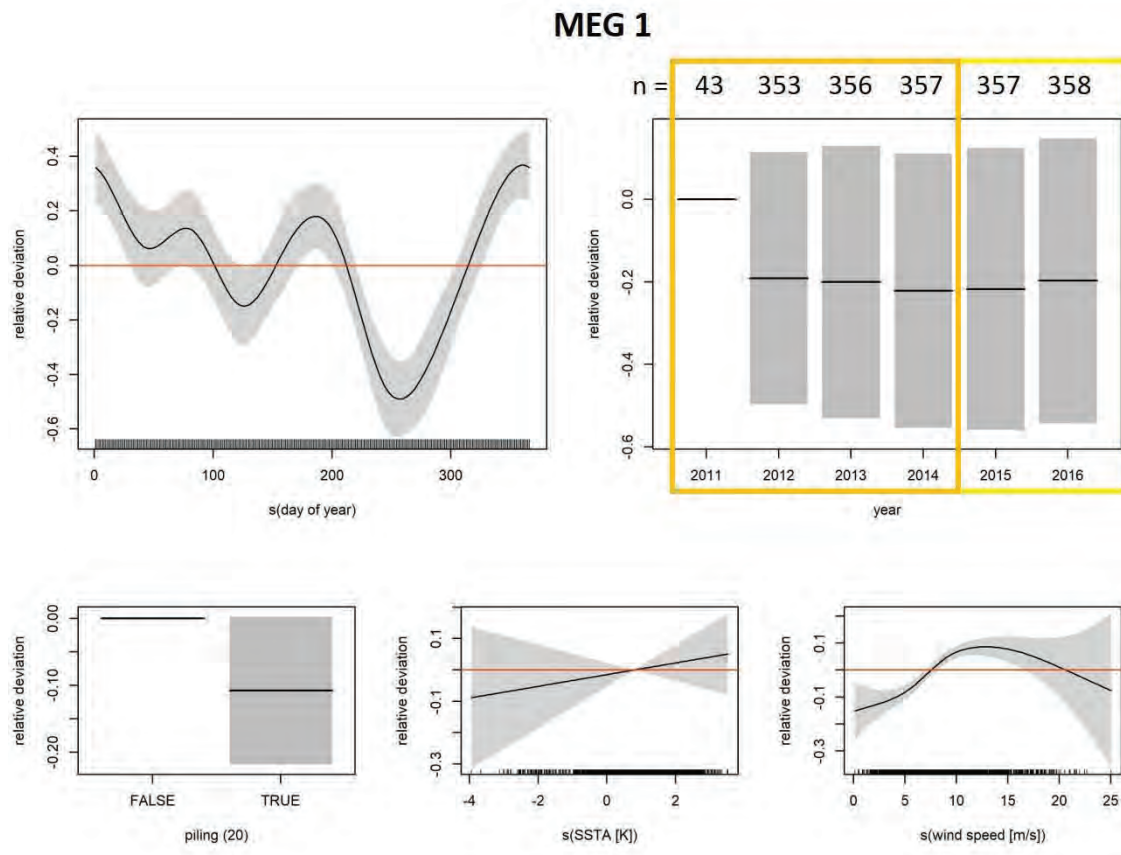
Figure 6.9 Effects of day of year, year, piling at a distance of 20 km, SSTa and wind speed on porpoise detection at the station MEG1. Grey-shaded areas indicate the confidence intervals. The number of recording days per year is indicated (n). Years in which piling occurred within a radius of 20 km to the monitoring station are marked with an orange box, years where piling occurred only within a radius of 50 km are marked with a yellow box.
