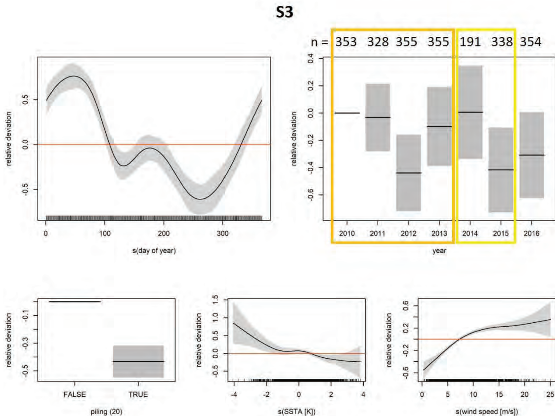
Figure 6.14 Effects of day of year, year, piling at a distance of 20 km, SSTa and wind speed on porpoise detection at the station S3. In 2016, station S3 was translocated some 1.9 km north and was called S3 new since. Data from the new station was included in this analysis. Grey-shaded areas indicate the confidence intervals. The number of recording days per year is indicated (n). Years in which piling occurred within a radius of 20 km to the monitoring station are marked with an orange box, years where piling occurred only within a radius of 50 km are marked with a yellow box.
