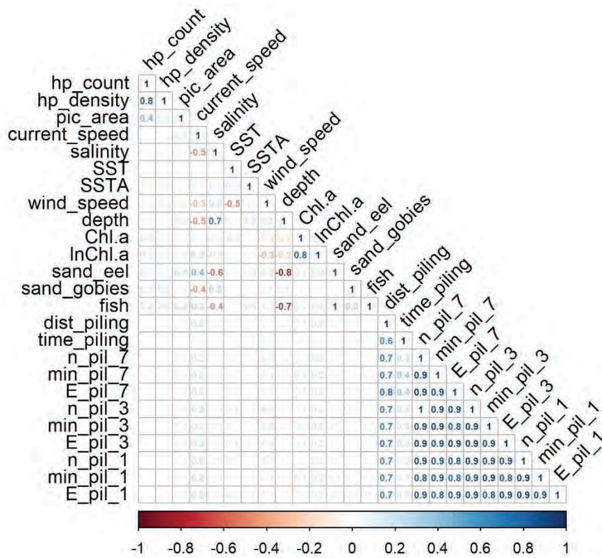
Figure 4.34 Correlation between explanatory variables for the complete dataset. Variables are explained in Table 4.15.
