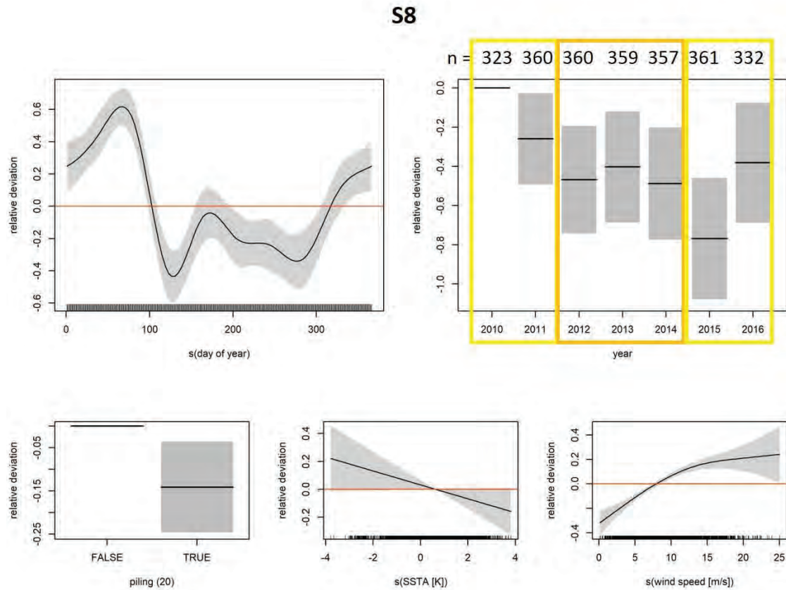
Figure 6.12 Effects of day of year, year, piling at a distance of 20 km, SSTa and wind speed on porpoise detection at the station S8. Grey-shaded areas indicate the confidence intervals. The number of recording days per year is indicated (n). Years in which piling occurred within a radius of 20 km to the monitoring station are marked with an orange box, years where piling occurred only within a radius of 50 km are marked with a yellow box.
