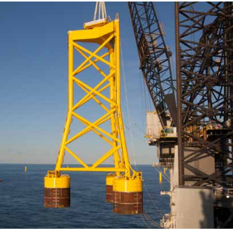
Figure 2: The three-legged SBJ installed at Borkum Riffgrund 1 by Ørsted
